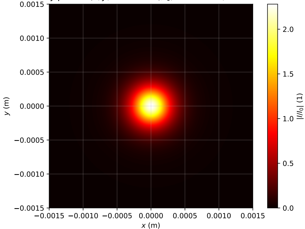
Intensity profile I(x, y, z = 2.309m)/I_0 , Pin=1.0Pcr, artificial time
